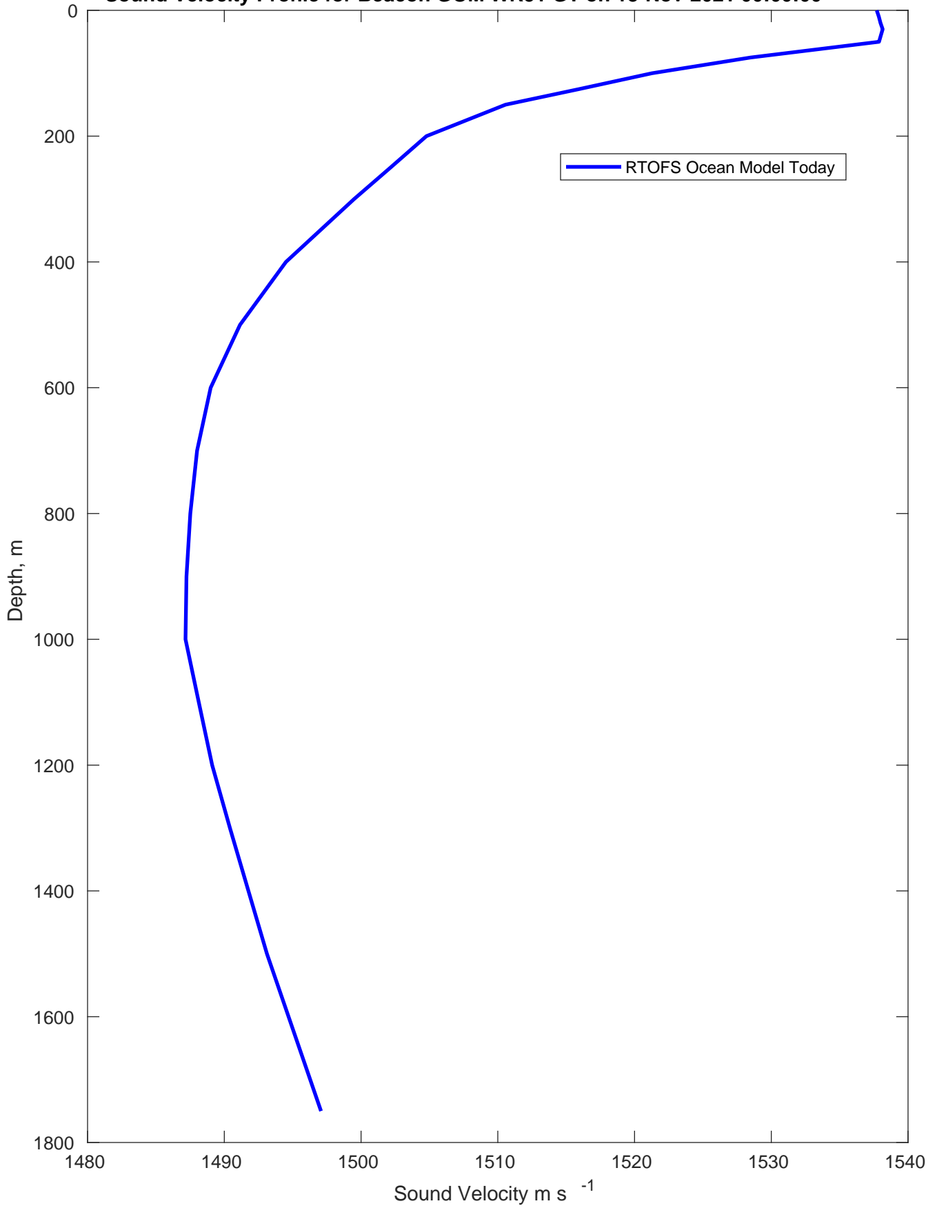
Sound Velocity Profile for Beacon GOM WR51 GT on 18-Nov-2021 00:00:00
